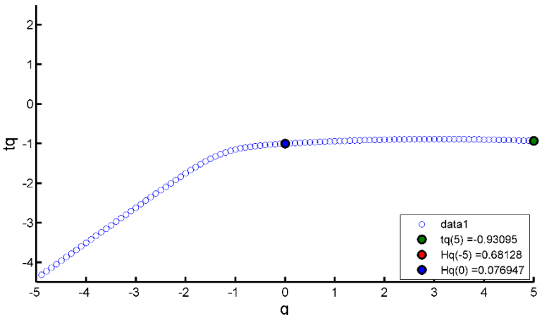
q-order Mass exponent
