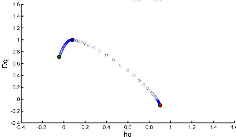
Multifractal spectrum ( h_{q_{\max}} - h_{q_{\min}} = 0.94554 )
