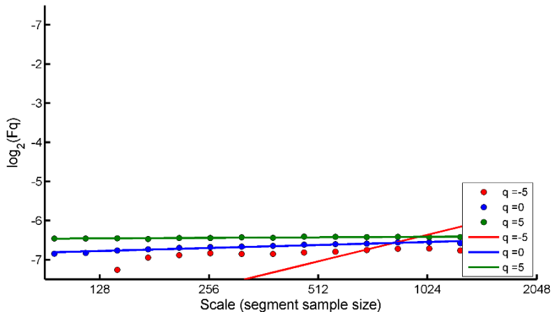
Scaling function F_q (q-order RMS with Slope = H_q )
