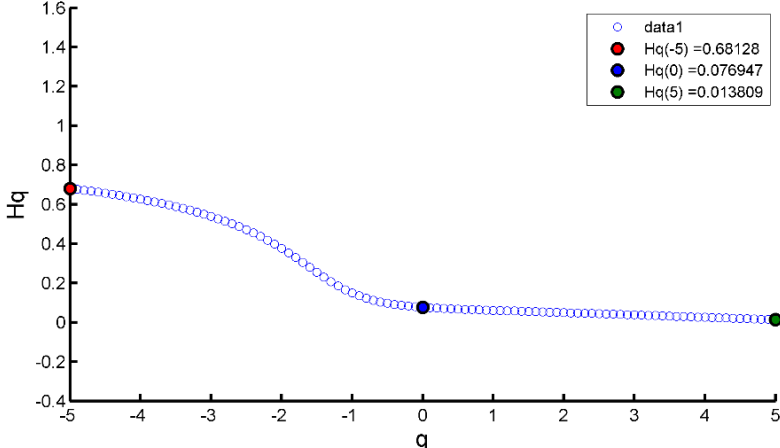
q-order Hurst exponent
